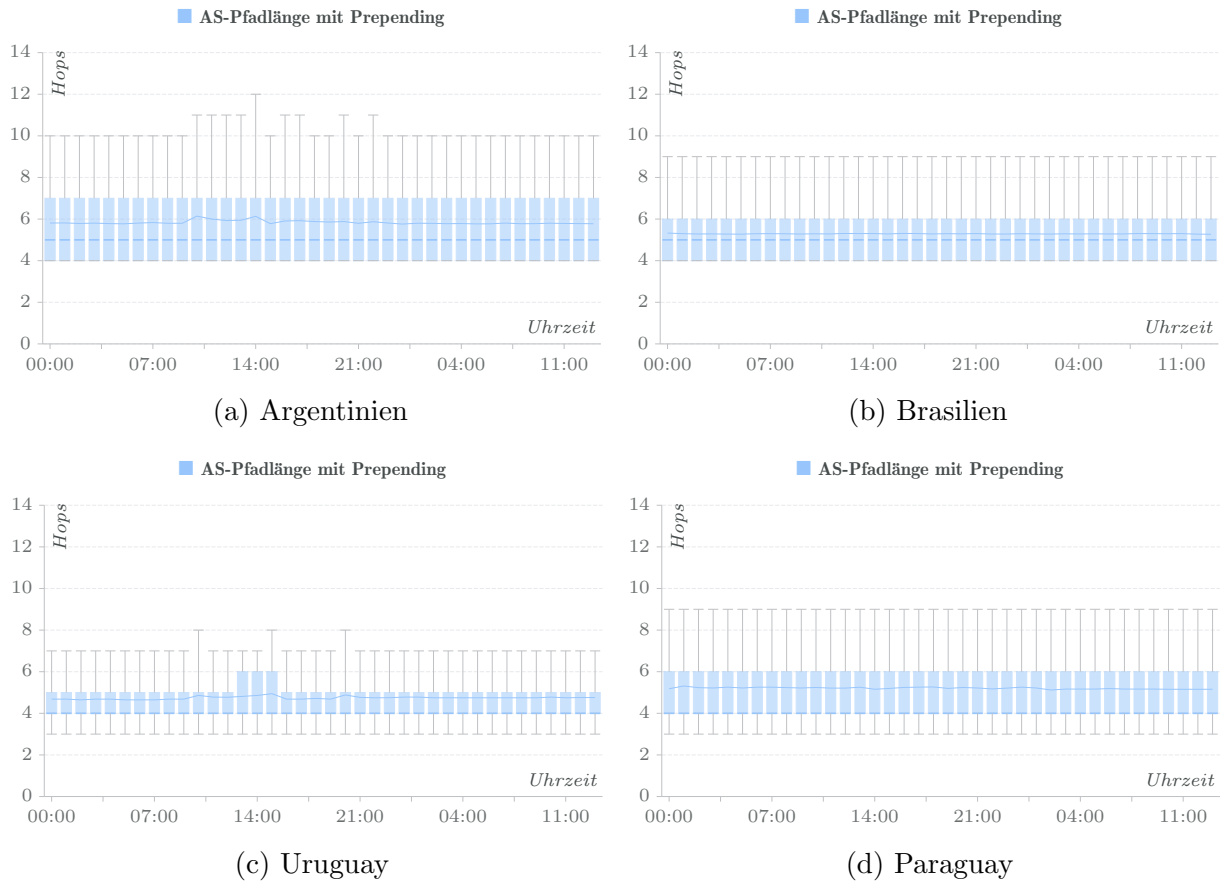
Abbildung 2.25: [I2] Pfadanalyse , inkl. AS Path Prepending (Control Plane)
